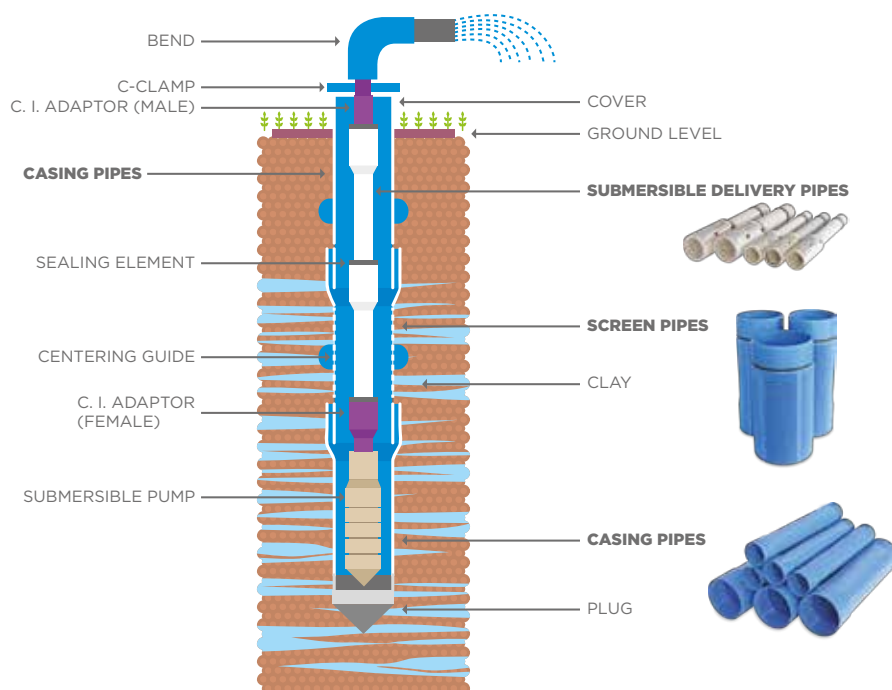
TYPICAL LAYOUT OF BOREWELL
